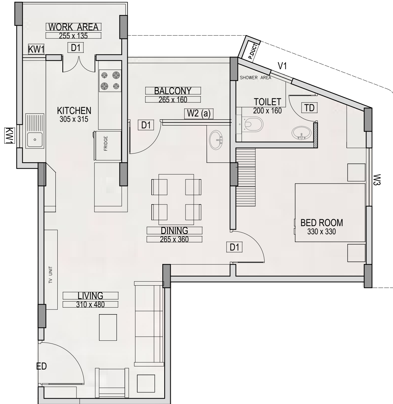
SECOND FLOOR
