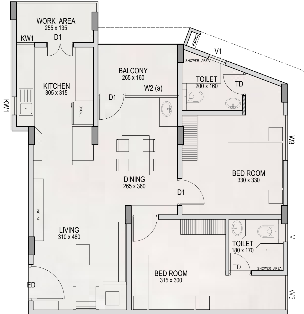
TYPICAL FIRST, THIRD & FOURTH FLOOR
