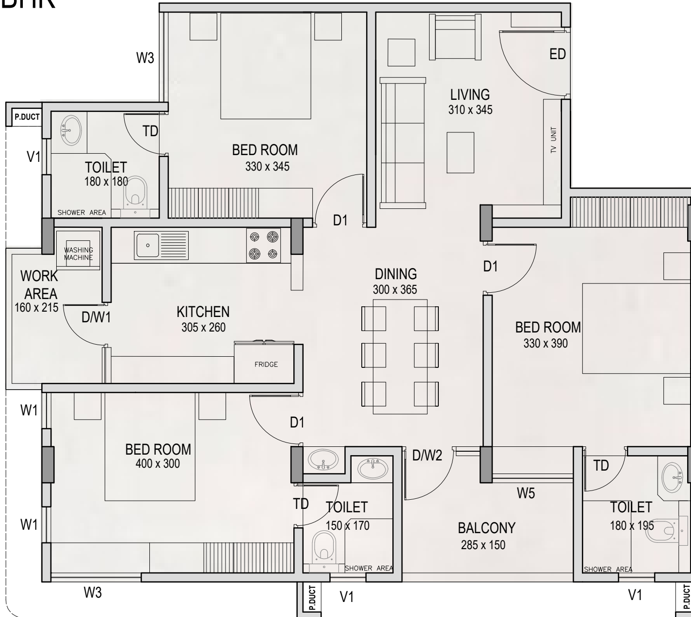
TYPICAL FIRST, SECOND, THIRD & FOURTH FLOOR
